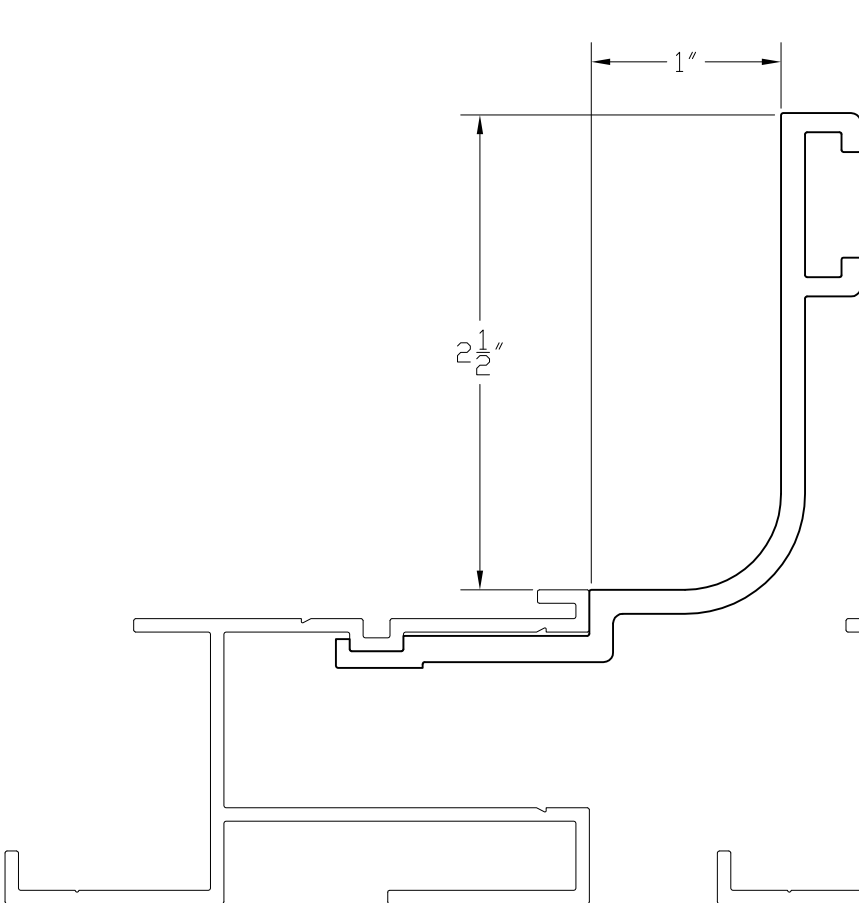
Cantilever Reusable Form
